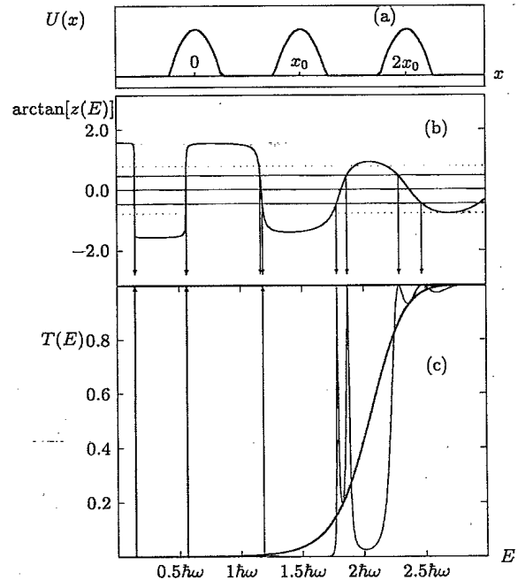
FIG. 4. Transmission coefficient for the periodic chain of three inverted parabolic barriers of frequency \omega . (a) Sketch of the potential. (b) Function z(E) determined by Eq. (79) of the text. Points of intersection of the z(E) graph with thin lines marked by vertical arrows are the graphical solutions of Eq. (86) and determine the positions of the transparency resonances. Points of intersection with dotted lines are the graphical solutions of Eq. (87) for the gap edges of semi-infinite chain. (c) Transmission coefficient T(E) for single barrier (bold line) and periodic chain (thin line). Resonances too narrow to be drawn on the figure are marked by vertical arrows.
