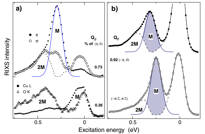
FIG. 2 (color online). (a) (top) RIXS spectra for \sigma and \pi polarization and Q_{\parallel} = 0.58 \text{ \AA}^{-1} along (100). The dashed line is the difference between the \pi spectrum and the Gaussian line shape ( M , solid blue line) representing the single-magnon contribution. (bottom) Comparison of Cu L -edge and O K -edge RIXS for Q_{\parallel} = 0.19 \text{ \AA}^{-1} . (b) RIXS spectra at 0.92(-\pi, 0) and (-\pi/2, \pi/2) measured with \sigma polarization. The two magnons ( 2M ) to single-magnon ( M ) intensity ratio is 0.26 at (-\pi/2, \pi/2) , and increases to 0.49 at 0.92(-\pi, 0) .
