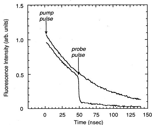
FIG. 6. Decay of the lowest-5d state in \text{Ce}^{3+} :YAG. The upper trace shows the decay following pulsed excitation at 500 nm. The lower trace shows the depopulation of the 5d state due to a strong 700-nm probe pulse at a 50-nsec time delay.
