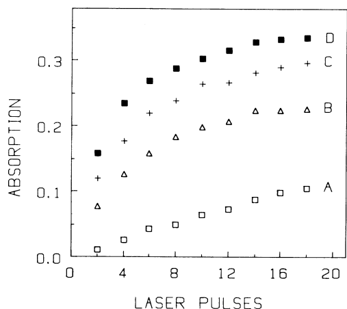
FIG. 4. The absorption ( \ln I_0/I ) of a 520-nm probe beam due to the growth of the divalent cerium color centers with accumulated exposure to the pulsed 308-nm laser. The laser intensities in \text{MW}/\text{cm}^2 are A, 10; B, 23; C, 33; D, 44.
