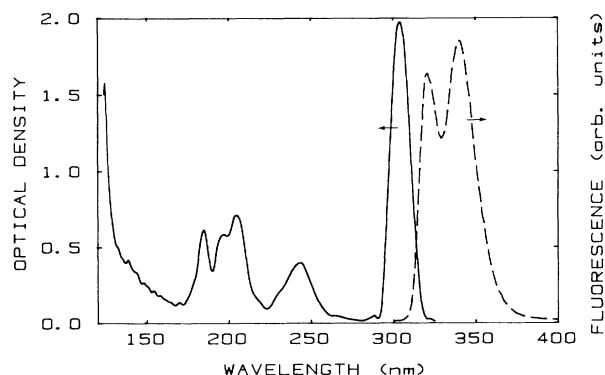
FIG. 1. Room-temperature optical absorption spectrum of 0.005% \text{Ce}^{3+}:\text{CaF}_2 (after Ref. 3) and the fluorescence spectrum following low-intensity 308-nm excitation.
