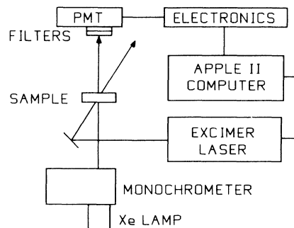
FIG. 3. Experimental apparatus used to investigate the spectral and growth characteristics of the color centers. The electronics used to interface the photomultiplier tube to the microcomputer include a current-to-voltage converter, a gated integrator, and a 12 bit analog-to-digital converter.
