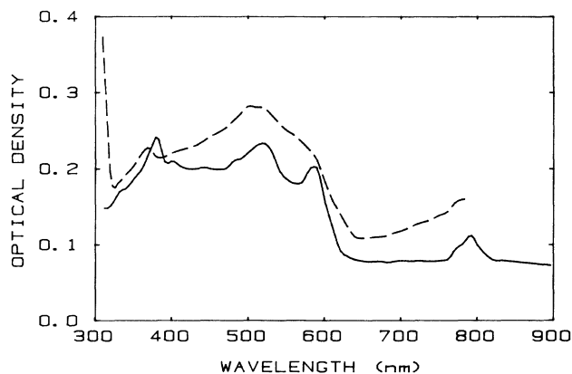
FIG. 2. Absorption spectra of the photochromic color center produced by the uv laser irradiation at 308 nm. Spectra are shown at 300 K (dashed curve) and 80 K (solid curve). The absorption bands are identified as those of divalent cerium.
