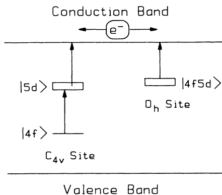
FIG. 7. Proposed model for the creation and bleaching of the photochromic center in \text{Ce}^{3+}:\text{CaF}_2 .
