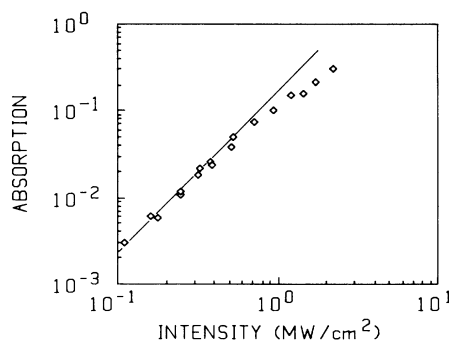
FIG. 6. Initial value of the change per laser pulse in the absorption of the 520-nm probe beam. The values for the lower intensity points depend quadratically on the laser intensity, as indicated by the straight line of slope 2.
