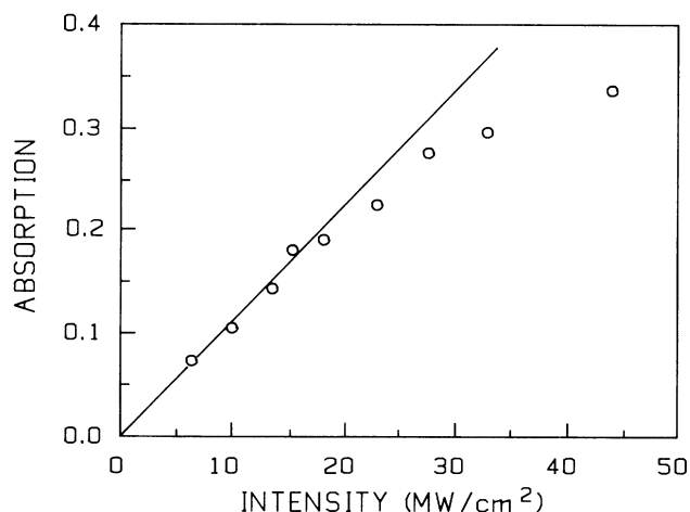
FIG. 5. Steady-state absorption ( \ln I_0/I ) at 520 nm due to presence of the divalent cerium color centers as a function of the peak intensity of the 308-nm laser. The straight line represents the linear approximation of Eq. (12).
