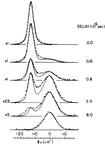
FIG. 4. Time-resolved emission spectra for the ^3P_0 \rightarrow (^3H_6)_1 fluorescence. The laser is pumping 12.0\text{ cm}^{-1} on the high-energy side of line center and the sample temperature is 14 K. The solid curves are the theoretical fit described in the text.
