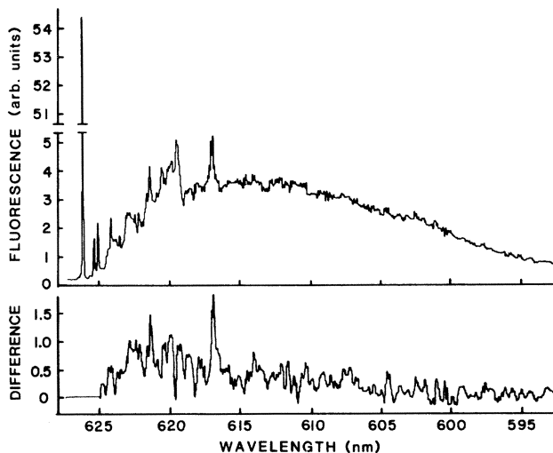
FIG. 8. Two-photon excitation spectrum where the laser is polarized at 45° to the [010] axis. The scale for the fluorescence intensity is the same as that in Fig. 3. The lower curve is the difference spectrum over the sideband and shows a wavelength-dependent polarization anisotropy.
