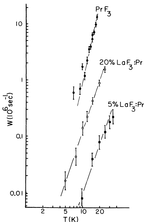
FIG. 12. Comparison of the spectral-transfer rates within the inhomogeneous ^3P_0 state for \text{PrF}_3 , 20% \text{LaF}_3\text{:Pr} , and 5% \text{LaF}_3\text{:Pr} .
