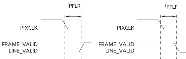
Figure 11: Propagation Delays for FRAME_VALID and LINE_VALID Signals
