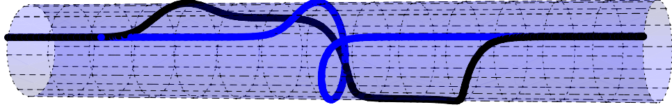
Figure 7. Same as Fig.5, but now for \mathbb{CP}^2 . Large instantons split into three Q = \frac{1}{3} kink-instantons, as the scale changes.
