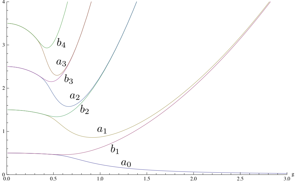
Figure 13. The energy eigenspectrum of the Mathieu equation as a function of g . For large- g^2 , it describes a particle with small moment of inertia I = 1/g^2 . The spectrum asymptotes to E_n = \frac{g^2}{2}n^2 . The small- g^2 regime is related to the Hamiltonian for \mathbb{CP}^1 in the Born-Oppenheimer approximation. The curves represent a_0, b_1, a_1, b_2, a_2, \dots , from (7.44), starting with the lowest curve. The mass gap E(b_1) - E(a_0) is a purely non-perturbative kink-instanton effect.
