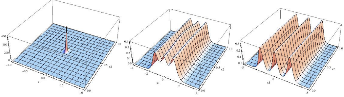
Figure 7. Same as Fig.5, but now for \mathbb{CP}^2 . Large instantons split into three Q = \frac{1}{3} kink-instantons, as the scale changes.
