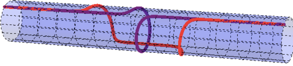
Figure 5. Small and large Q = 1 instantons in \mathbb{CP}^1 in a weak coupling center-symmetric background. Large instantons split into two Q = \frac{1}{2} instantons.
