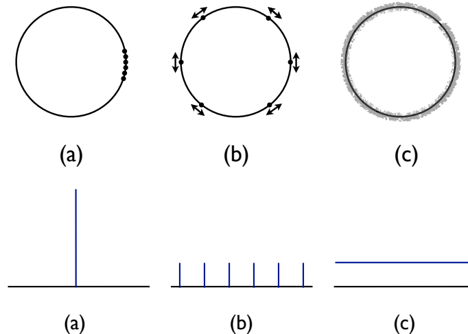
Figure 1. Three types of gauge holonomy in non-abelian gauge theories and analogously \sigma -connection holonomy (defined in (2.34)) in non-linear sigma models, and their classification according to their eigenvalue distribution. a) is the weak coupling trivial holonomy. b) and c) are, respectively, the weak and strong coupling non-trivial holonomy, and they are continuously connected in the sense of gauge invariant order parameters. In b), the eigenvalues of holonomy are located at the roots of unity and their fluctuations are small. In c), the positions of the eigenvalues are uniform and randomized. In gauge theory on \mathbb{R}^3 \times S^1 , b) is the counterpart of the weak coupling adjoint Higgs regime. There is no weak coupling or even a potential description for c). The difference between (b) and (c) in gauge theory is discussed in Ref. [12].
