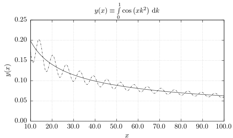
Figure 7: Asymptotics Eq. (58) (dashed line) and Eq. (61) (solid line) compared to numerically evaluated Eq. (57) (dotted line) for 10 \leq x \leq 100 .
