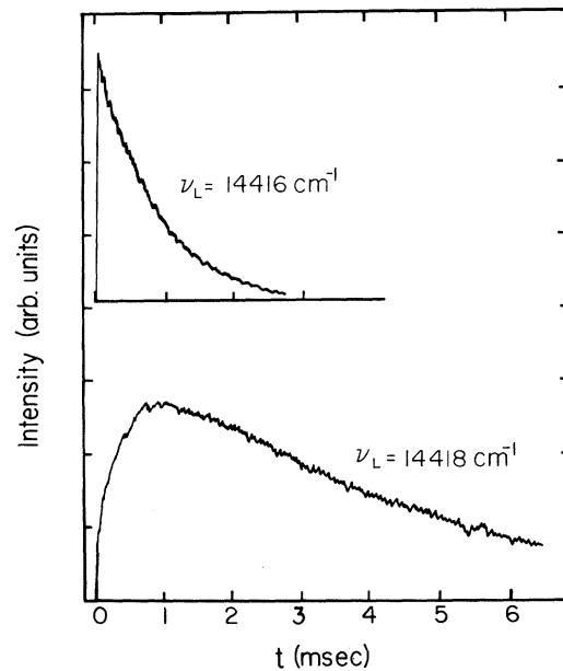
FIG. 3. Time-resolved studies for the 7009-Å N -line fluorescence in a 0.51-at.% sample at 5 K. Upper trace obtained when pumping directly into N -line absorption, lower trace when exciting center of R_1 absorption.
