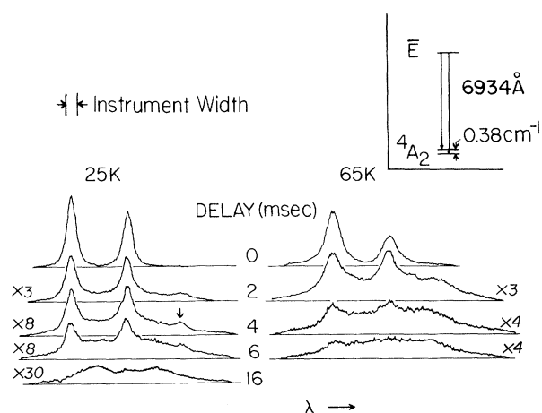
FIG. 1. Typical time-resolved studies for a 0.2-at.% ruby sample at two different temperatures, with the integrated intensities scaled to roughly the same value. Gain settings relative to the 0-delay traces are shown. Inset shows the R_1 fluorescence transitions involved. Below 40 K, the width of the narrowed components reflects the instrumental profile. The peak separation is 0.38 \text{ cm}^{-1} , and the third peak indicated by an arrow is a radiative transfer effect, to be discussed in a subsequent article.
