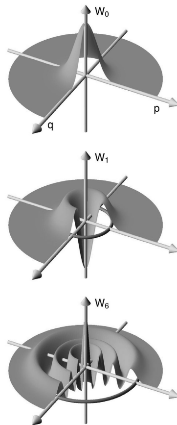
Fig. 1. Gallery of Wigner functions of a single mode of the radiation field. The Wigner function of the vacuum (top) is always positive whereas the ones corresponding to a single photon (center) or six photons (bottom) contain significant domains where the phase space distribution assumes negative values. The circle visible in the quadrant of the foreground indicates where the phase space trajectory corresponding to the energy \hbar\Omega(n+1/2) runs. The scales on the axes are identical in all three cases.
