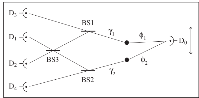
Fig. 6. Quantum eraser – One of two atoms (solid circles) emits two photons \phi_i and \gamma_i . Interference is observed in \phi by scanning detector D_0 . Beamsplitters BS1 – BS3 direct \gamma to four detectors. A click in detectors D_3 or D_4 provides which-path information on \gamma , preventing interference in \phi . A click in detectors D_1 or D_2 erases which-path information and restores interference in \phi . Figure adapted from Ref. [29].
